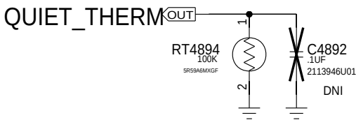
QUIET TEMP SENSOR
