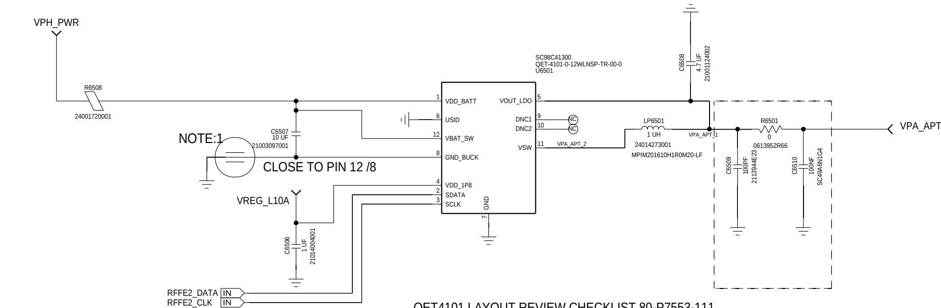
QET4101 LAYOUT REVIEW CHECKLIST 80-P7553-111
