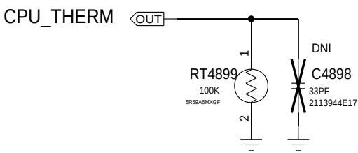
FOR SM7150 THERMAL
