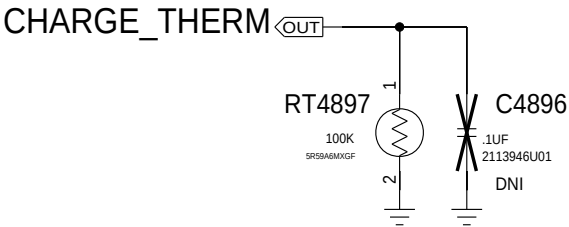
CHRG TEMP SENSOR
